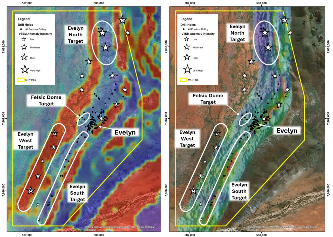
Figure 2: Electro-magnetic anomalies generated from 200m-line spaced VTEM survey over regional Airborne Magnetics (left) and Ground Magnetics (right). MGA Zone 50
